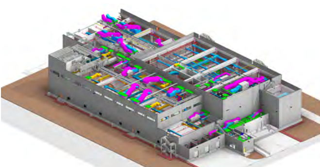
BIM Model of Factory
